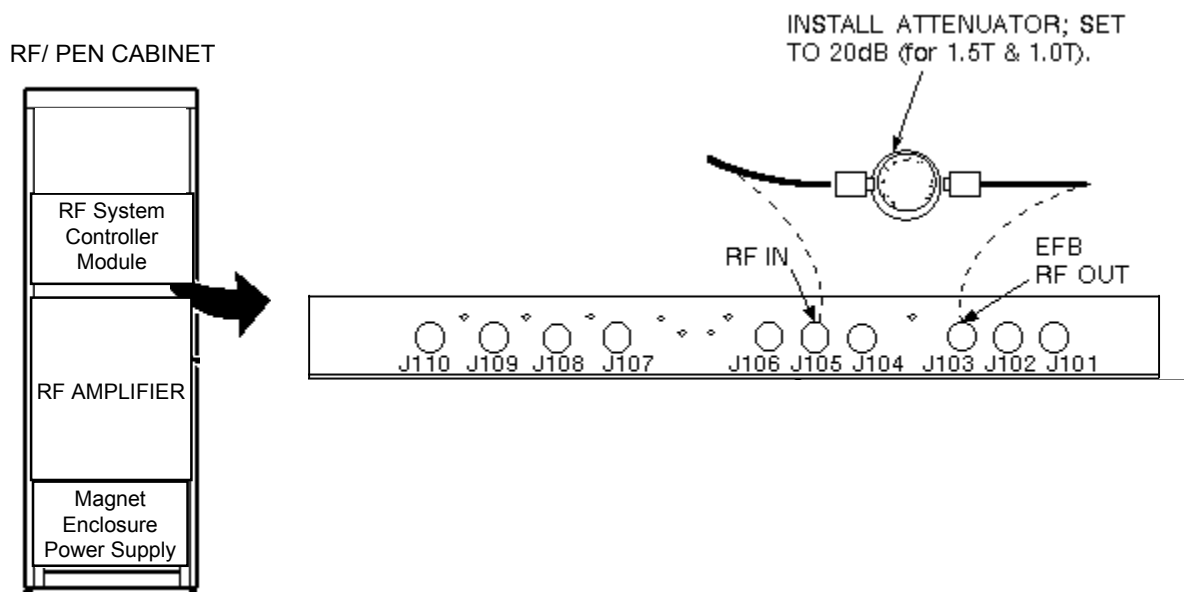
RF/PEN CABINET: RF SYSTEM CONTROL MODULE WITH EFB BYPASSED ILLUSTRATION 5-4A
