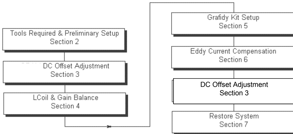
GRAM/SGA TUNING & GRAFIDY FLOWCHART ILLUSTRATION 1-1
