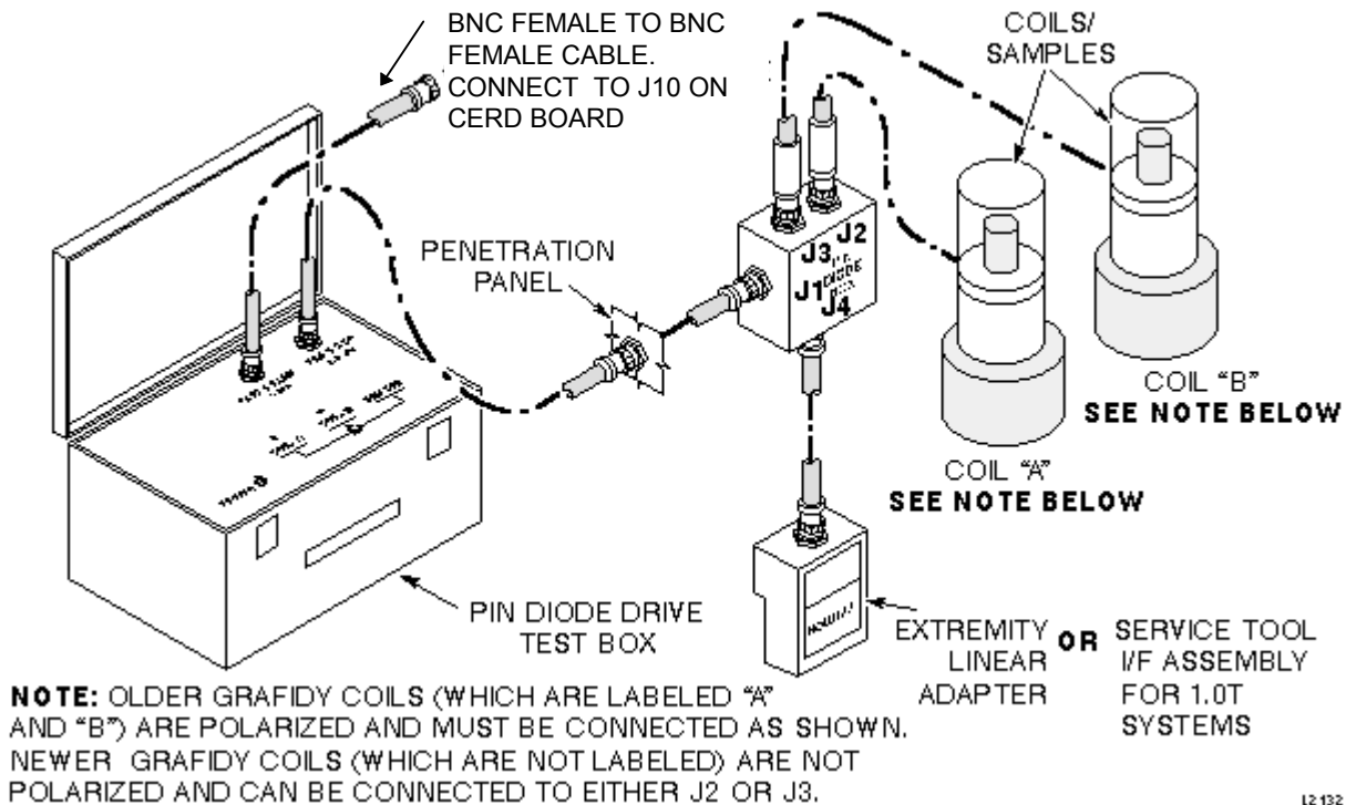
GRAFIDY KIT SETUP ILLUSTRATION 5-2
